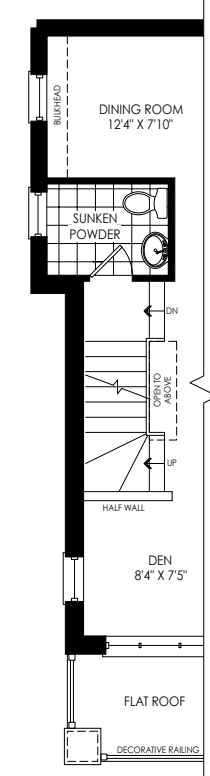
ELEVATION BF, BH
